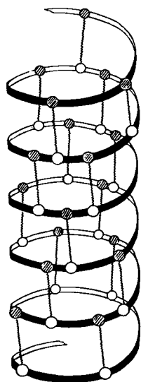
FIGURE 2 Illustration of an \alpha -helix where \circ denotes peptide oxygen, and \odot peptide nitrogen, and \sim\sim\sim denotes hydrogen bond.
